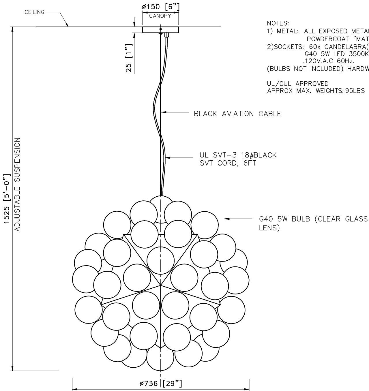
FRONT VIEW
